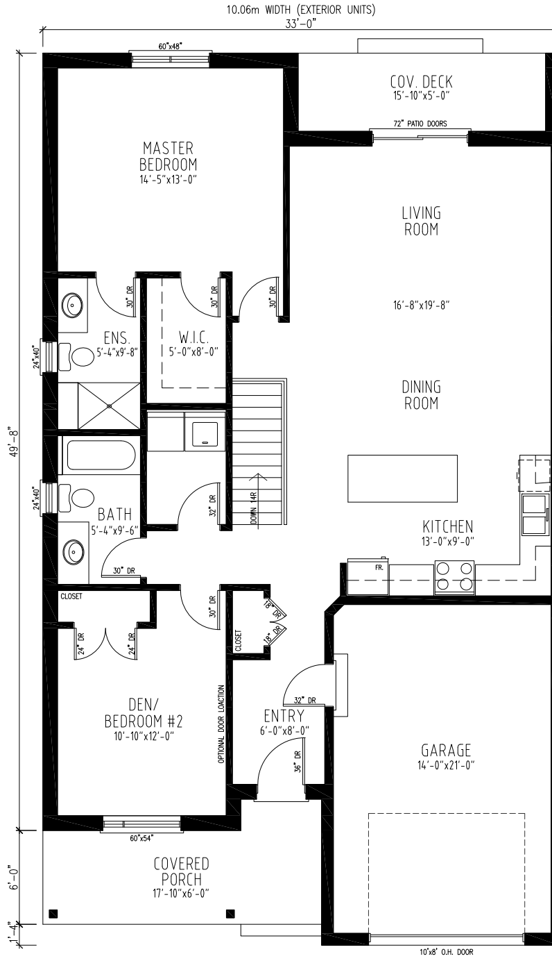
MAIN FLOOR PLAN EXTERIOR BUNGALOW 1336 S.F.
