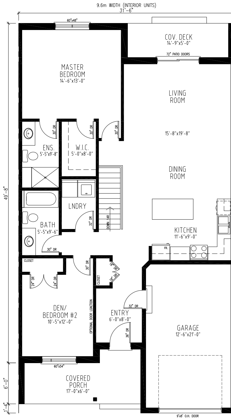
MAIN FLOOR PLAN INTERIOR BUNGALOW 1286 S.F.
