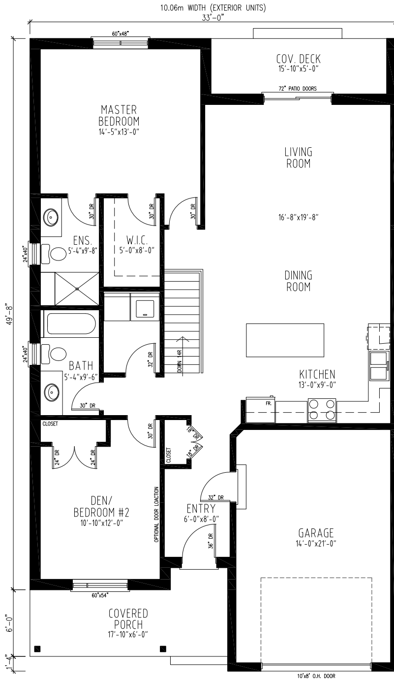
MAIN FLOOR PLAN EXTERIOR BUNGALOW 1336 S.F.
