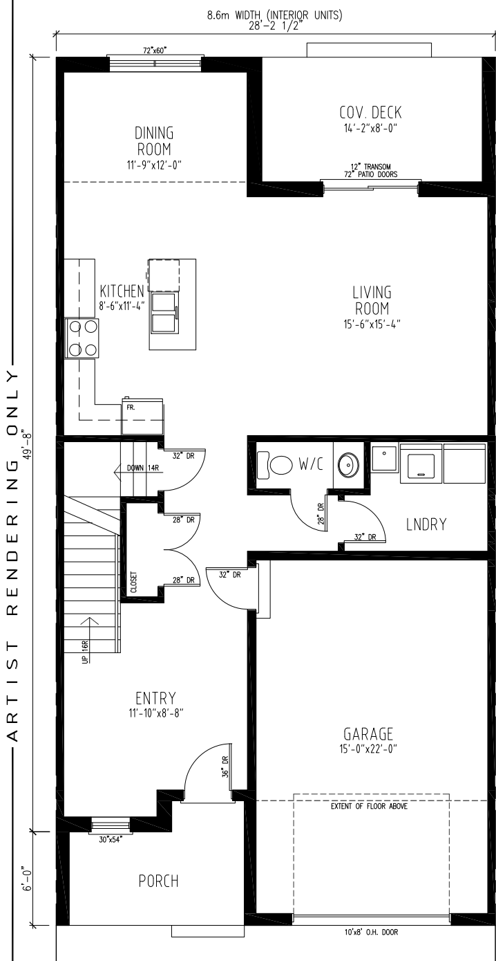
FIRST FLOOR PLAN INTERIOR TWO STOREY 1000 S.F.
