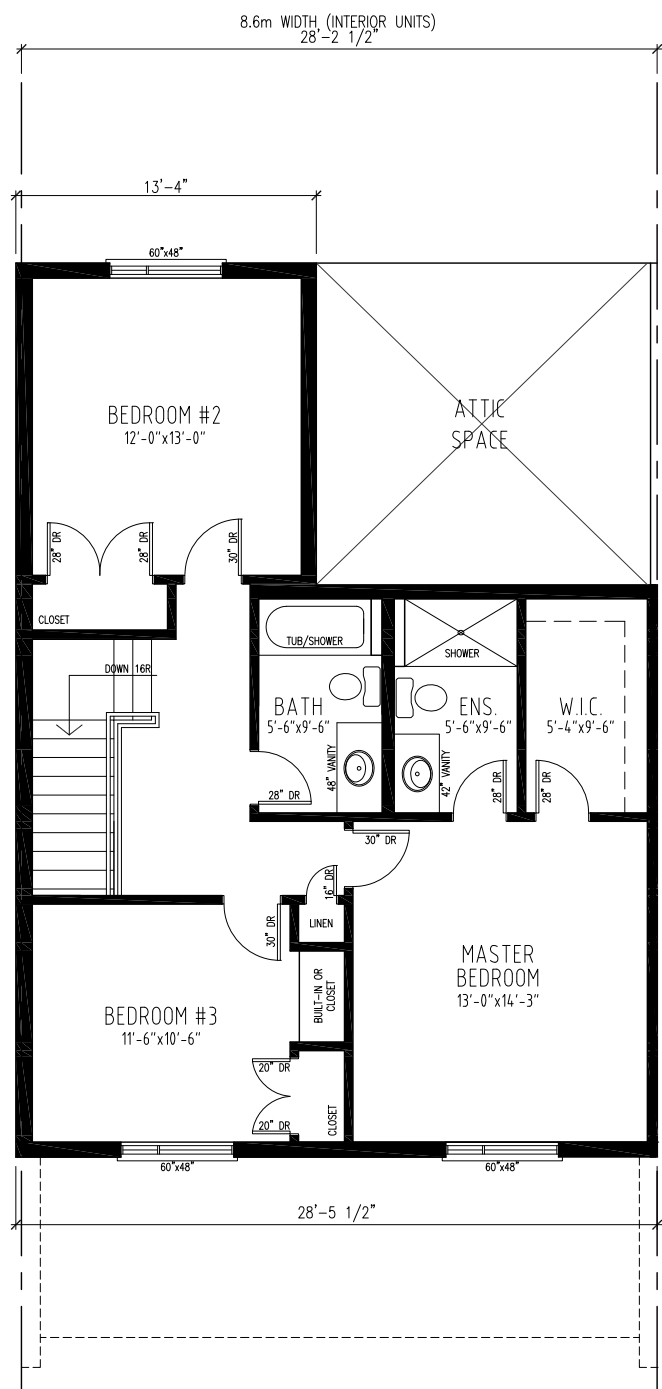
SECOND FLOOR PLAN INTERIOR TWO STOREY 844 S.F.
