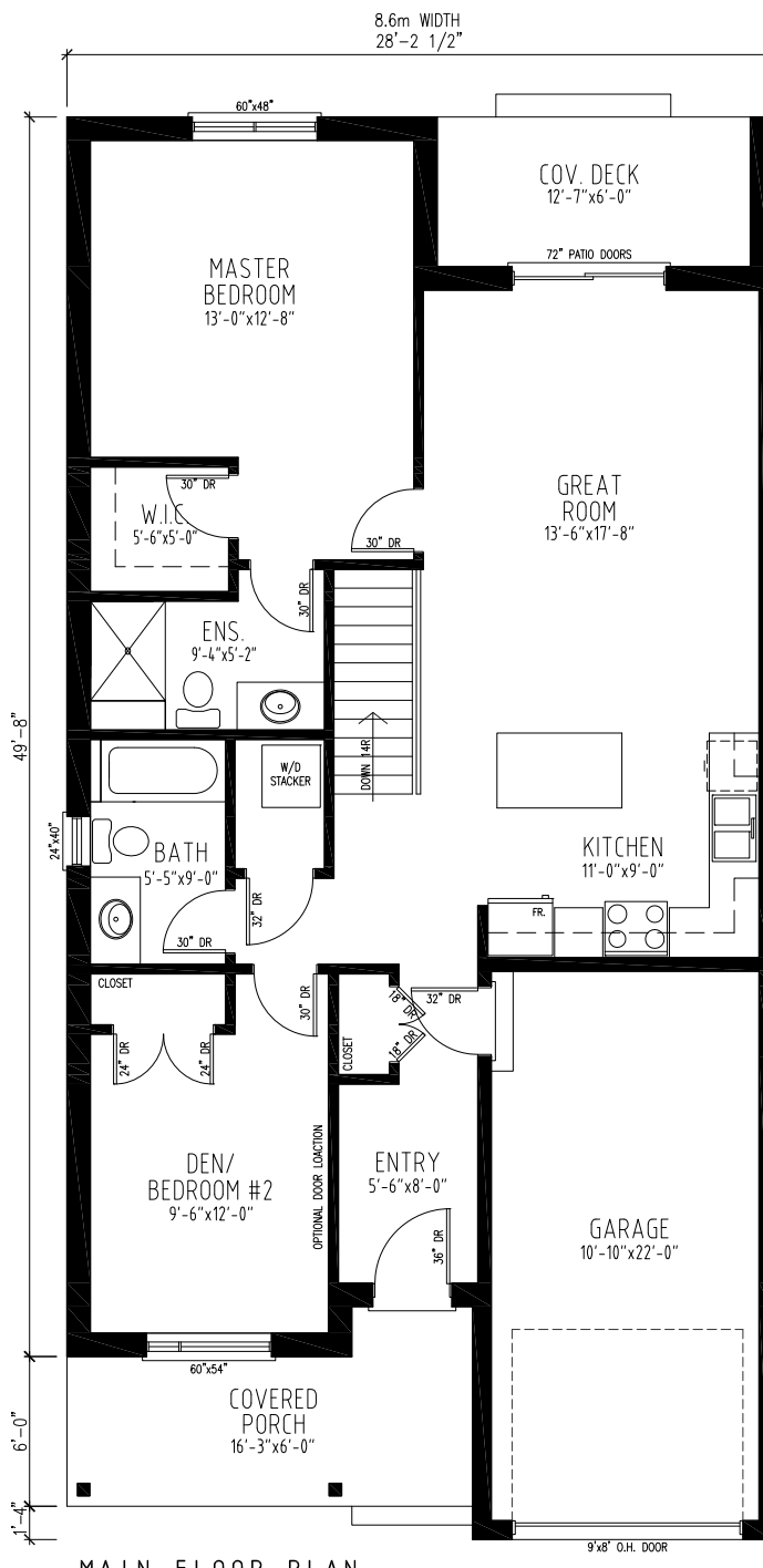
MAIN FLOOR PLAN SMALL EXTERIOR BUNGALOW 1136 S.F.
